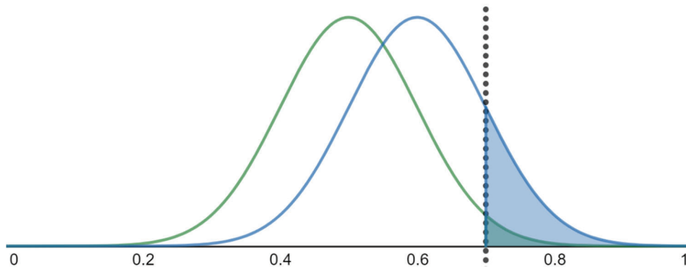
Figure 1. Score distribution of Green and Blue groups: different mean.
