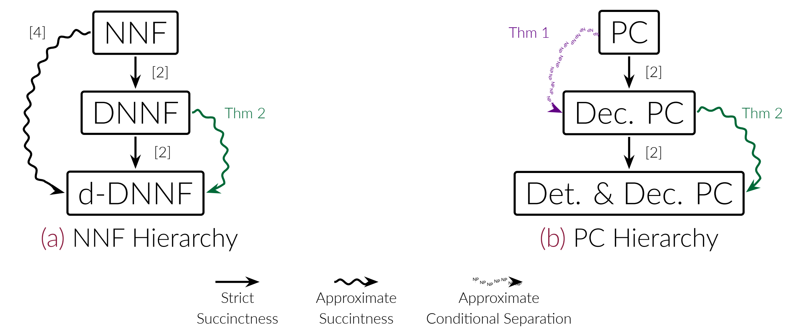
Figure: Updated succinctness relationships for NNF and PCs.
